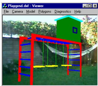
Real-time software
